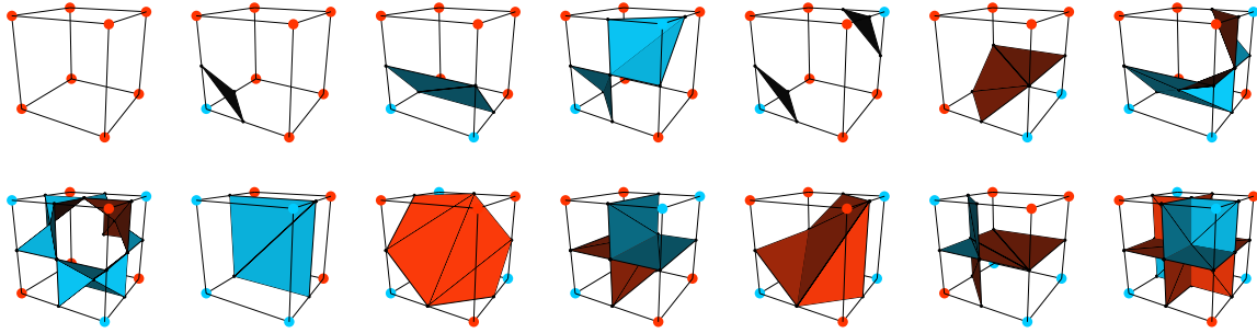
Figure 6: If the field function can be classified into three regions or less, the initial triangles in the MC cell are generated using a look-up table which has been created by symmetrically modifying the look-up table for the original marching cubes algorithm. The triangles can be modified and removed according to the field values assigned to the MC vertices. This figure shows the look-up table used in our method for binary classification, which is a portion of the table proposed in [12]
