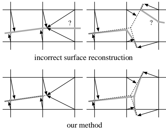
Figure 2: The upper left shows an example of incorrect surface reconstruction due to the discontinuity of the surface connection, which has been corrected by preventing unnecessary interpolation in the lower left. The upper right shows another example of incorrect reconstruction due to the ambiguity of surface orientation. This problem is caused by binary classification of the distance field, and is successfully solved by considering multiple classification by introducing the segmented distance field which is explained in section 3.3.
