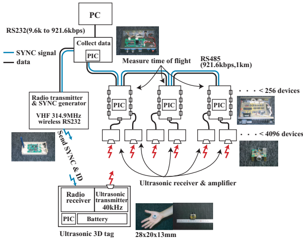
Fig.3 System configuration
