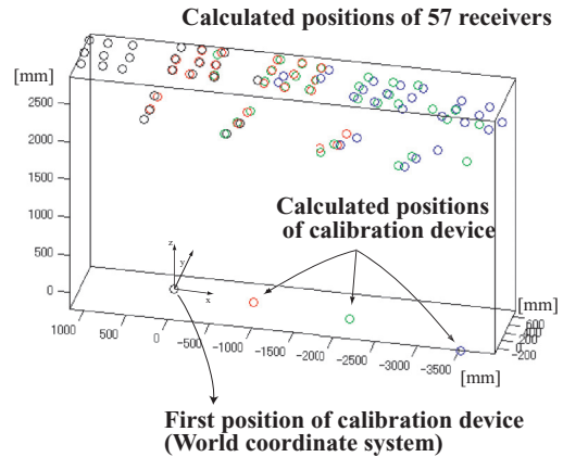
Fig.5 Experimental result
