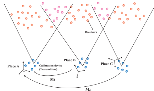
Fig.2 Calibration method
